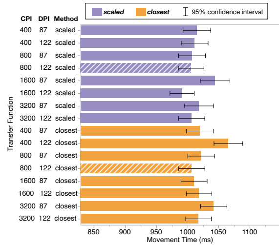
Figure 4: Overall Mean Movement Time (Y) for each TRANSFER FUNCTION (X). The baseline function is highlighted with hatching.
