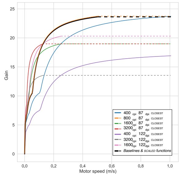
Figure 3: Gain functions used in the experiment, expressed in gain (Y, unitless) per physical unit (X, m/s). The functions of the form A_{CPI}B_{DPI}CLOSEST are represented in physical units using Equation (1) with R_i = A/25.4 , R_o = B/25.4 , and T_i = 8 ms. Both baseline conditions (800 CPI 122 DPI SCALED, 800 CPI 122 DPI CLOSEST) and all SCALED functions are superimposed (black line). Transfer functions in libpointing are expressed in accordance with the HID standard, which encodes input signal in 8-bit integers and is therefore limited to 127 levels [3, p.61]. For higher input values, we maintained the highest gain value of each function (dotted lines).
